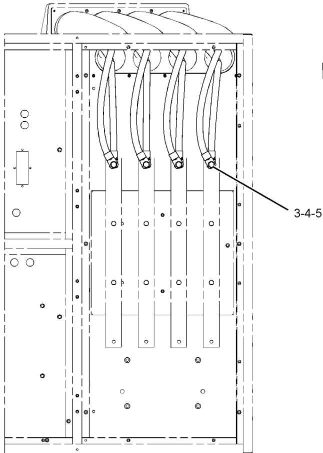
REAR VIEW
