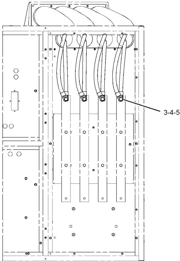
REAR VIEW
