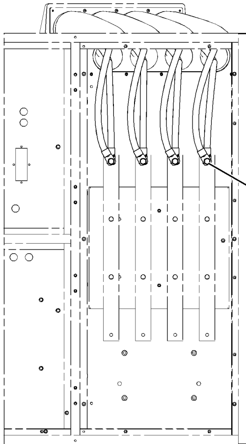
REAR VIEW
